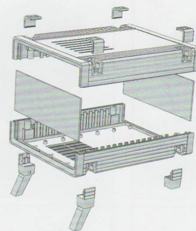
装配图(Assembly drawing)
