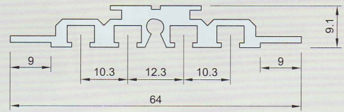
连接板 Connecting board
