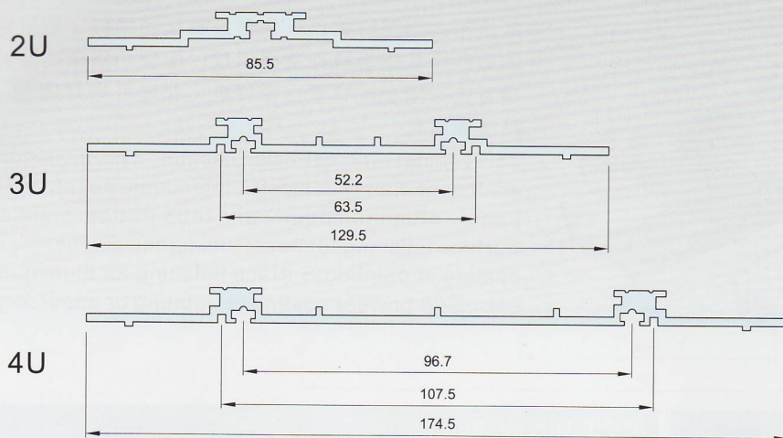
后横梁(Rear beam)
