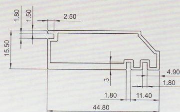
侧梁(Side beam)
