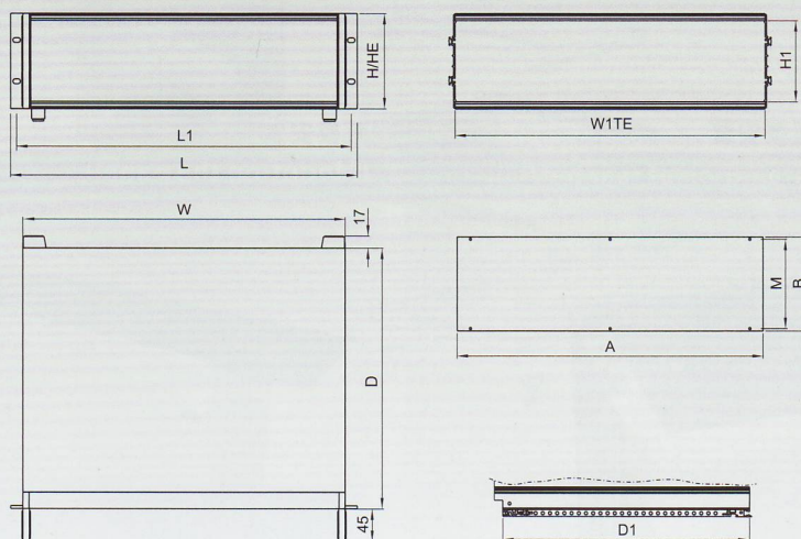
尺寸图(Dimension)
