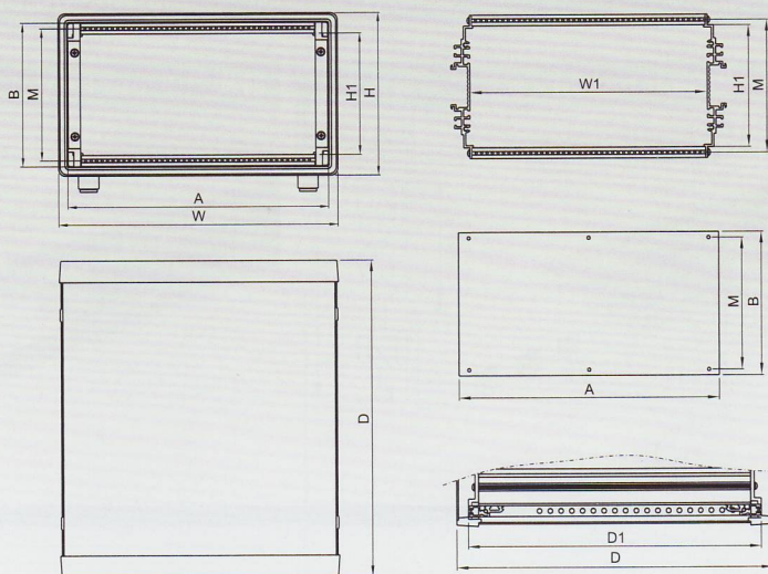
尺寸图(Dimension)
