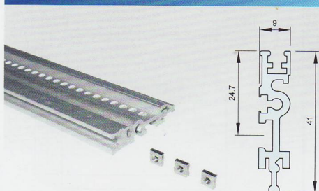
后横梁(Rear beam)
