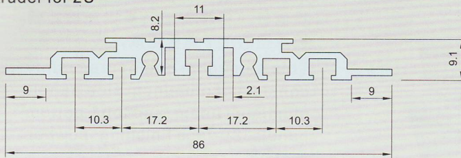
2U型材 Extruder for 2U
