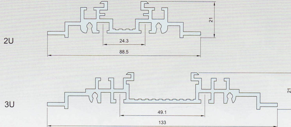
螺母条(Tapped strip)
