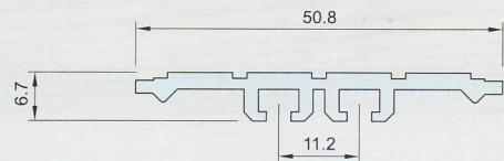
连接板 Connecting board
