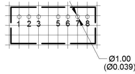
印刷版俯视图 Printed board vertical view
