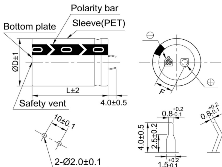
(PC board hole dimensions) (Terminal dimensions)
