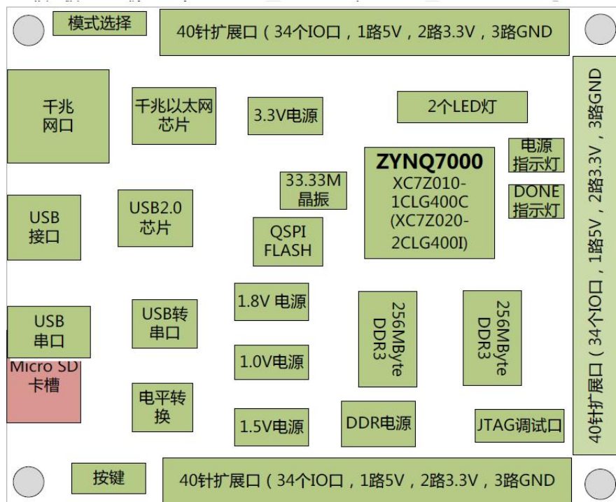
Figure 1-1: The Schematic Diagram of the AC7010C/AC7020C
