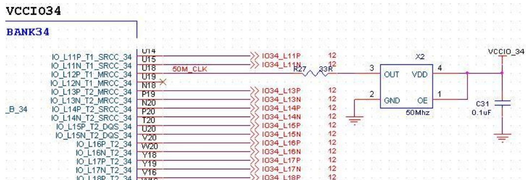
Figure 5-3: PL system clock source
