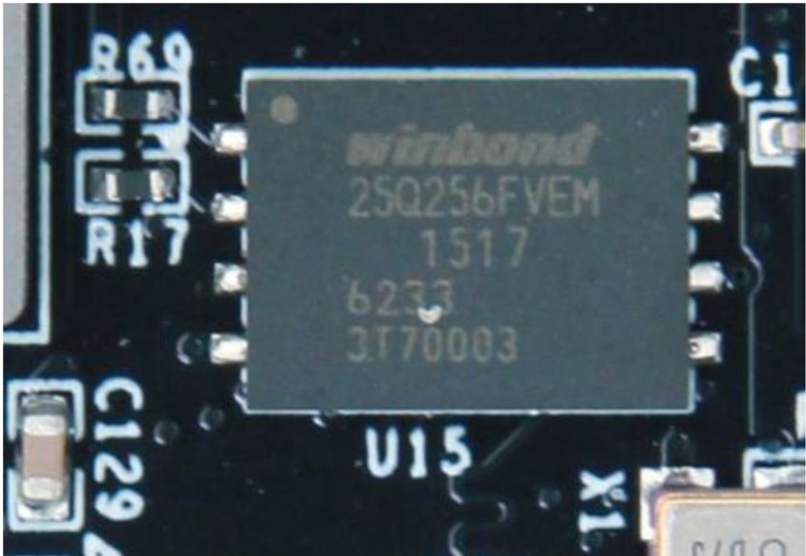
Figure 6-2: QSPI Flash on AC7010C/AC7020C FPGA Core Board
