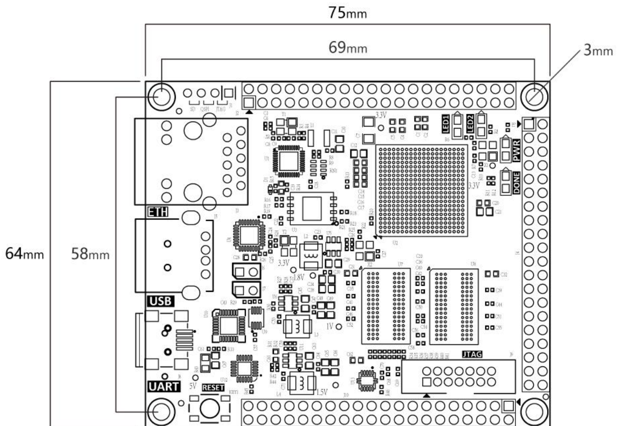
Figure 2-1: FPGA Size Dimension
