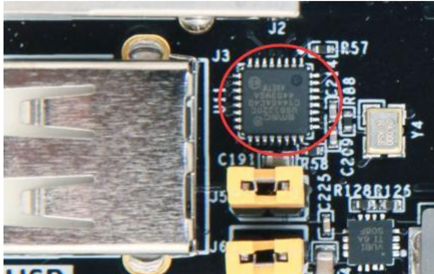
Figure 6-7: The USB3320C chip on the FPGA Board
