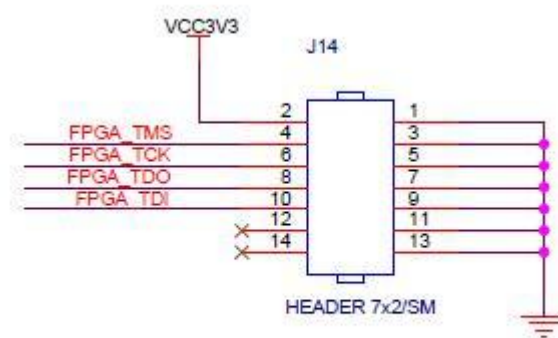
Figure 4-3: The JTAG port schematic
