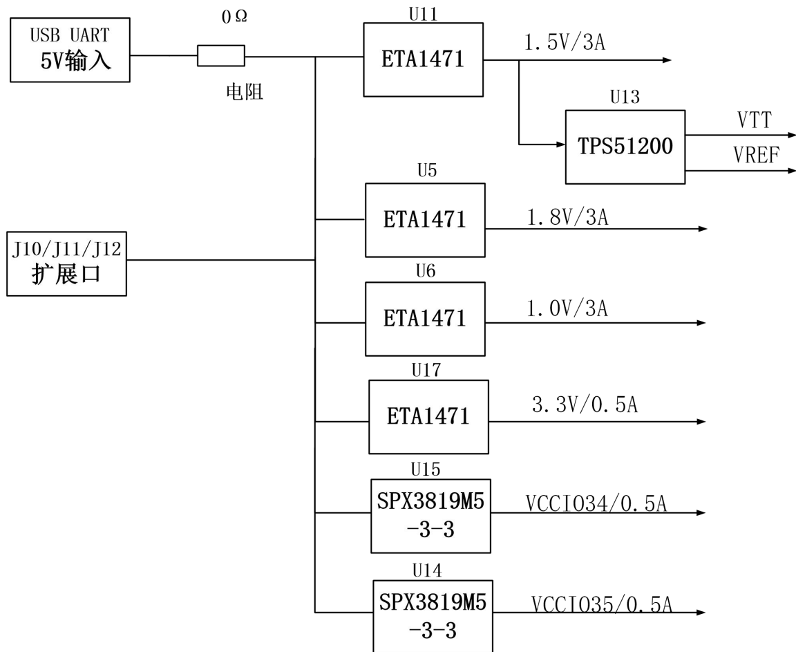
Figure 3-1: Power Supply Schematic
