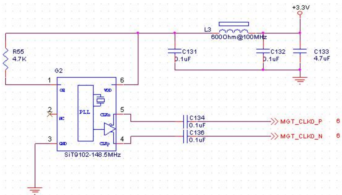
Figure 3-3: 148.5Mhz Active Differential Crystal Schematic
