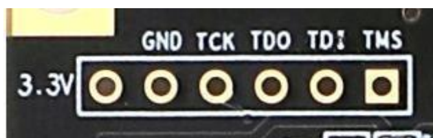
Figure 7-2 JTAG Interface on Core Board
