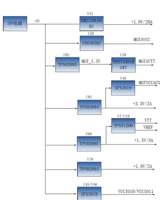
Figure 9-1: Power interface section in the schematic
