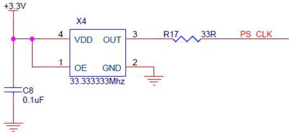
Figure 6-2: Active crystal oscillator to the PS section
