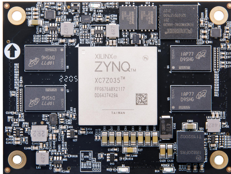
Figure 1-1: AC7Z100C Core Board (Front View)
