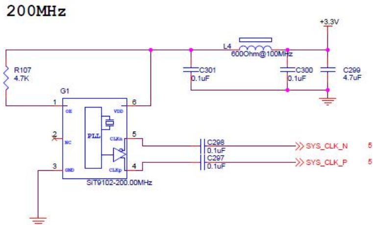
Figure 6-3: PL system clock source
