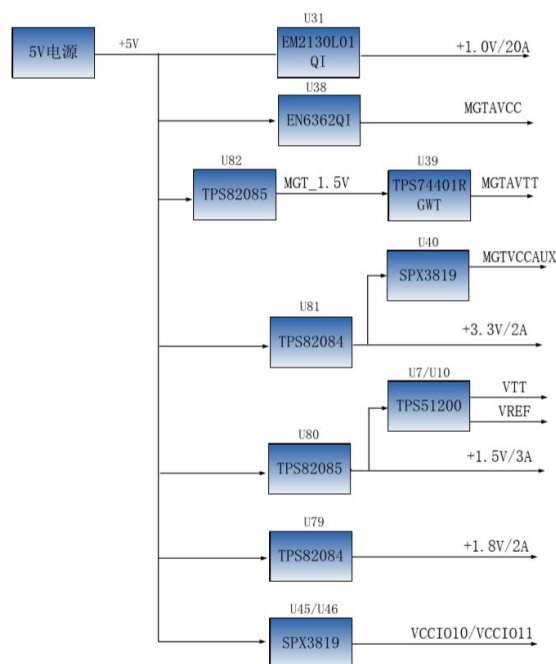
Figure 9-1: Power interface section in the schematic
