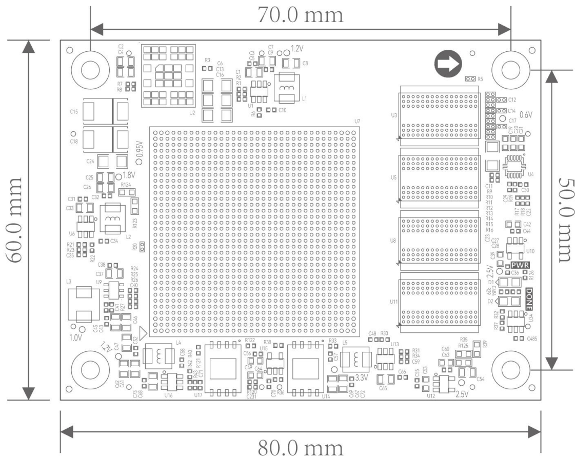
Figure 8-1: (Top View)
