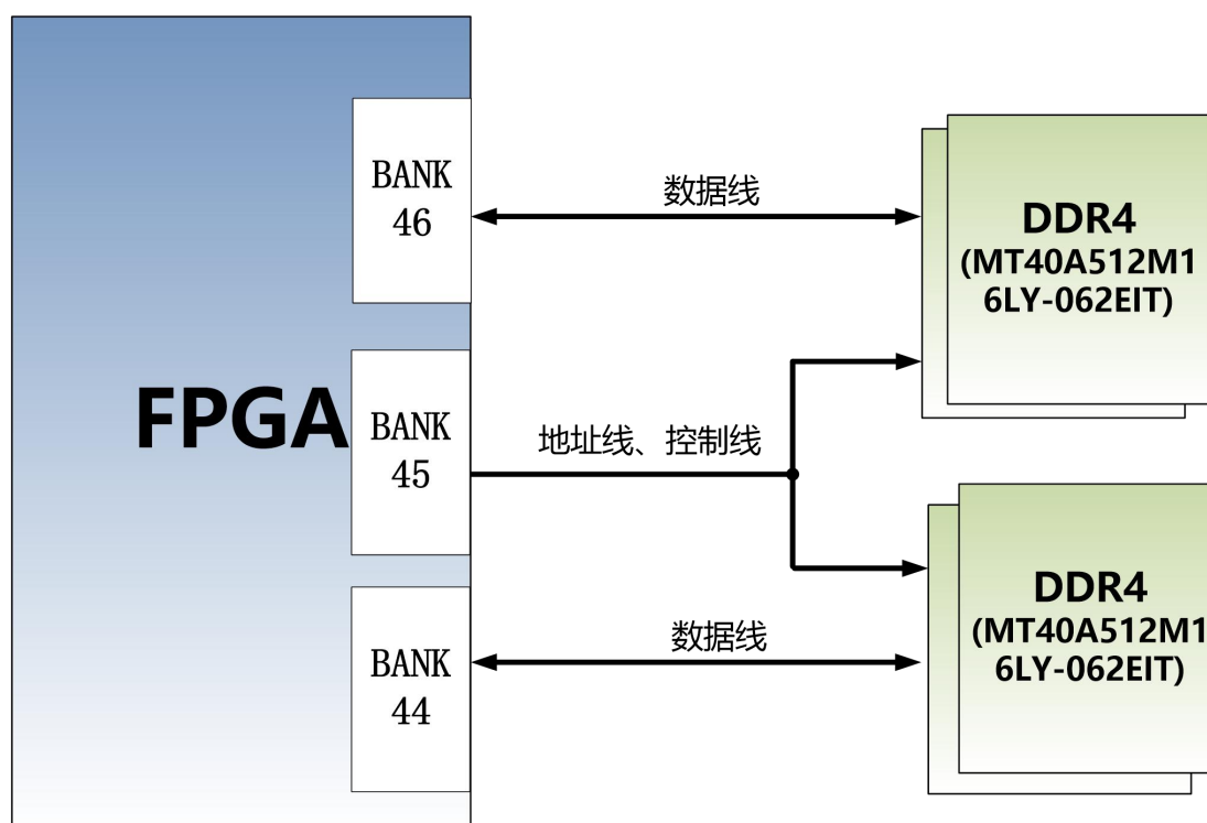
Figure 1-3-1 DDR4 DRAM Schematic
