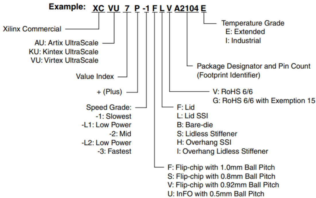
Figure 2: Ordering Information
