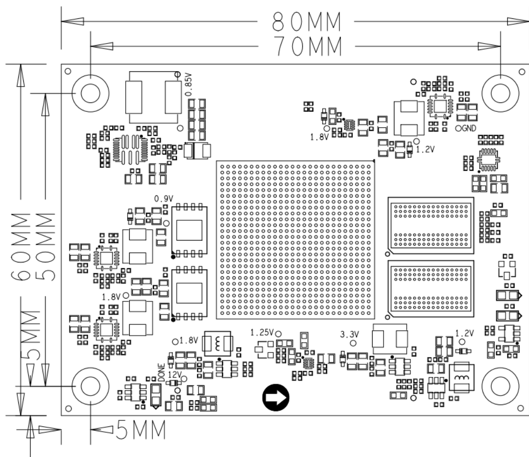
Figure 2-8-1 Top View
