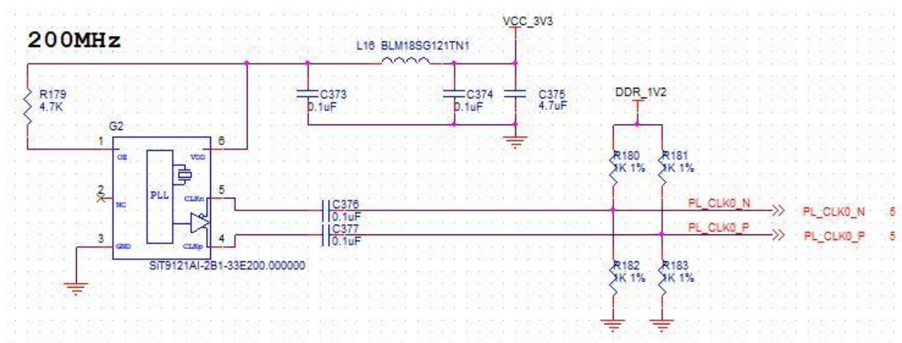
Figure 1-6-4: PL system clock source
