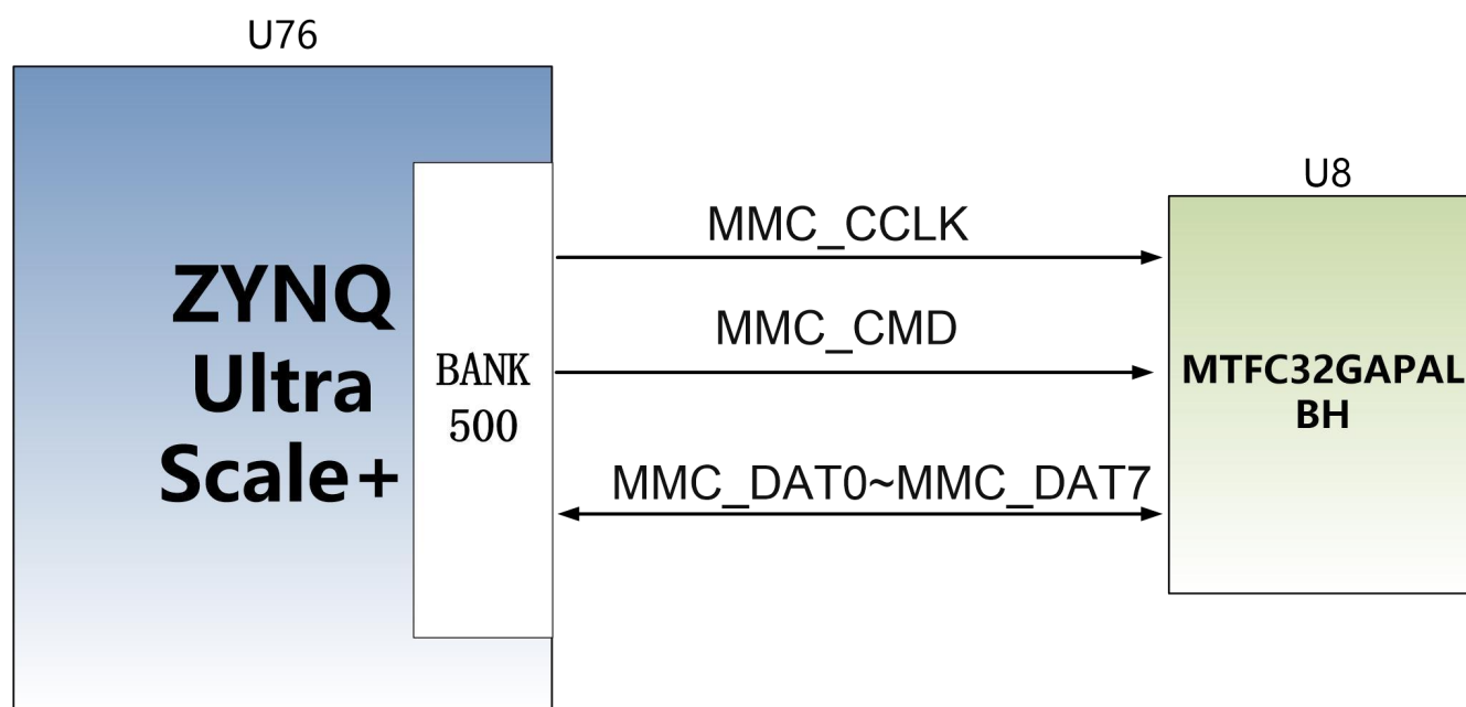
Figure 1-5-1: eMMC Flash in the schematic
