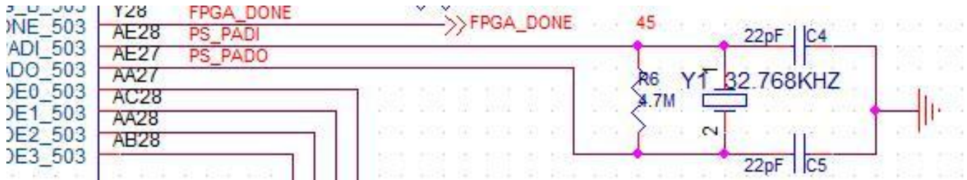
Figure 1-6-2: Passive Crystal Oscillator for RTC
