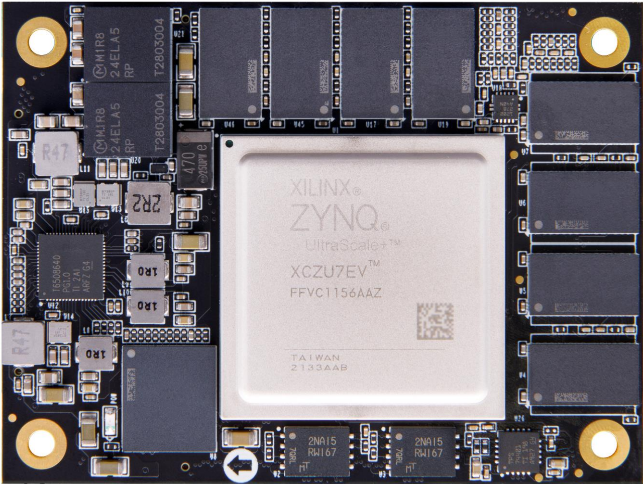
Figure 2-1-1: ACU7EVC Core Board (Front View)
