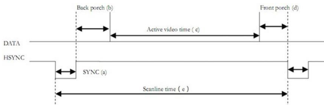
Figure 3-8: VGA Time Timing
