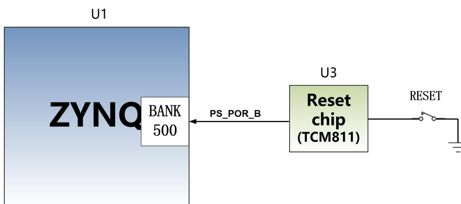
Figure 2-9-1: Reset button connection diagram
