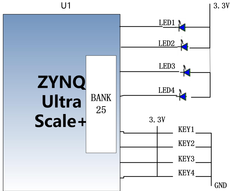
Figure 17-1: LED Schematic
