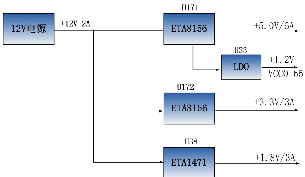
Figure 3-22-1: Power supply interfaces in schematic diagram
