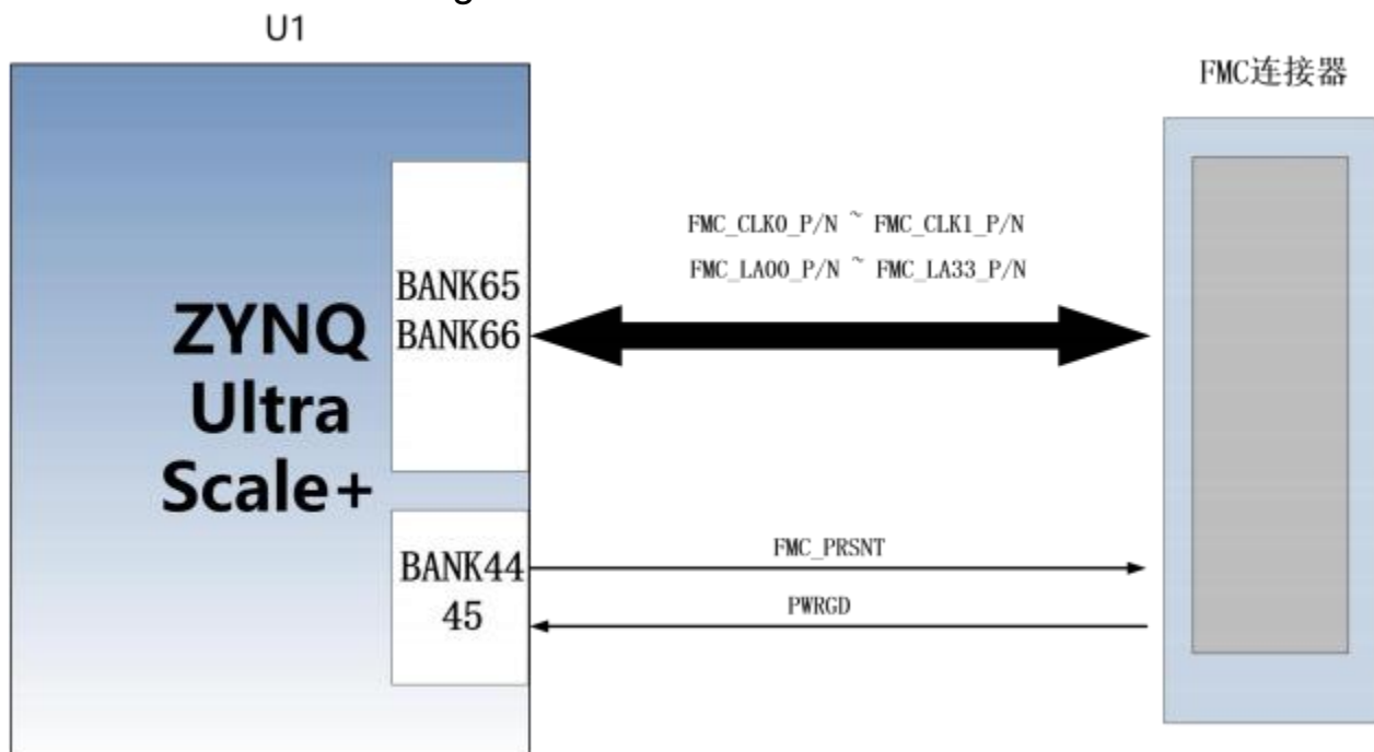
Figure 3-15-1: FMC Schematic
