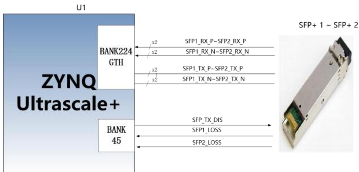
Figure 3-10-1: SFP Schematic
