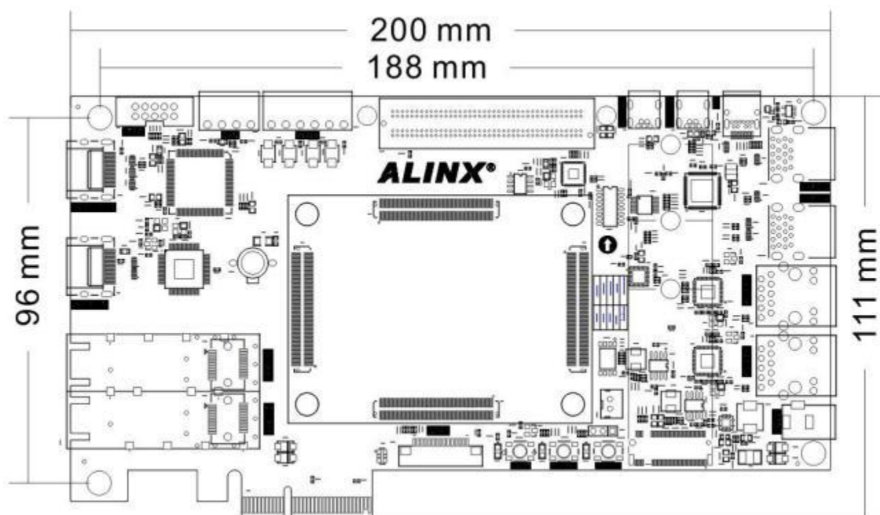
Figure 3-24-1: Top View
