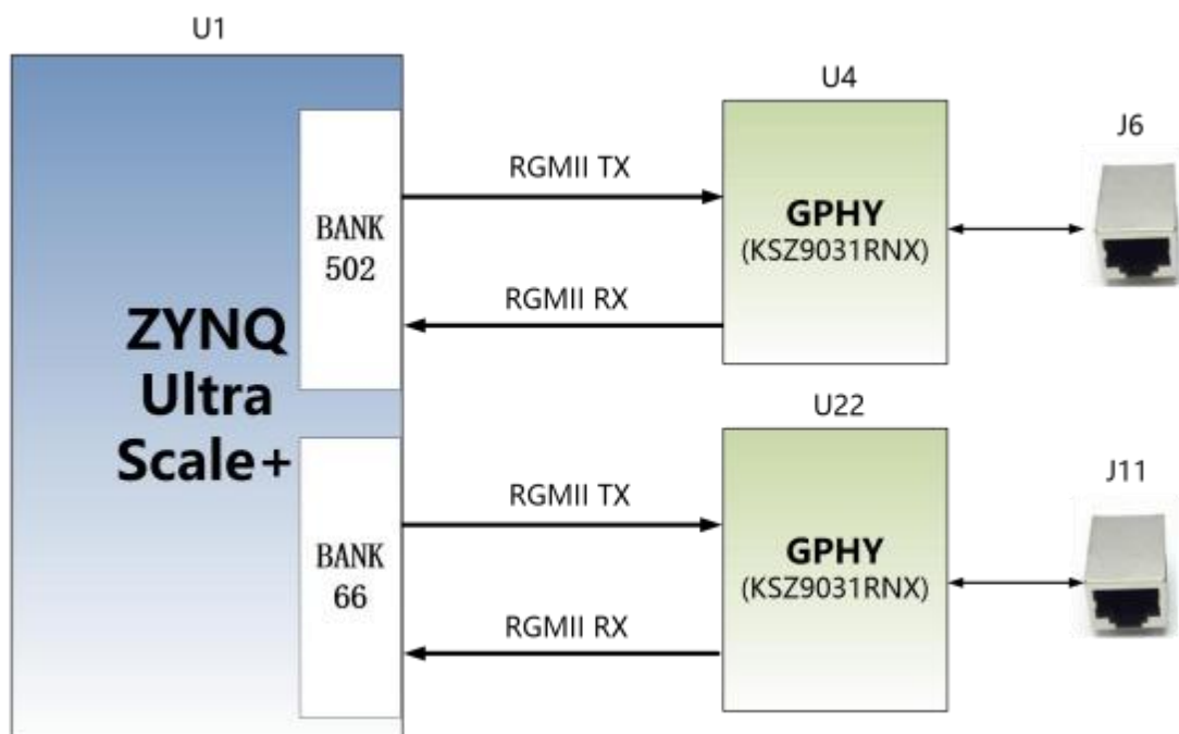
Figure 3-5-1: Connection diagram of ZYNQ and GPHY
