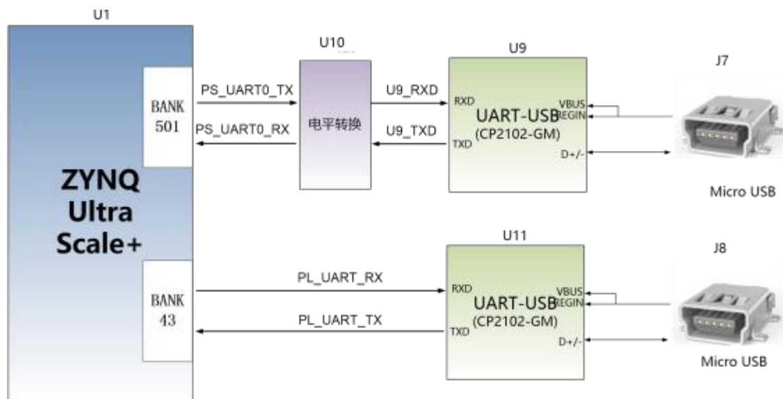
Figure 3-6-1: USB to serial port schematic
