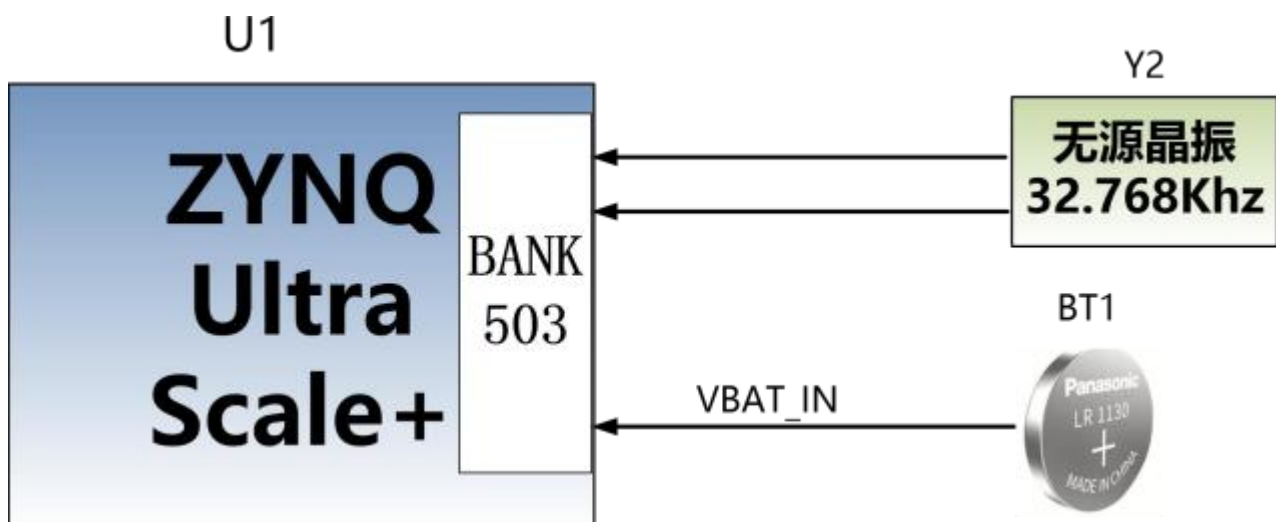
Figure 3-17-1: RTC Schematic
