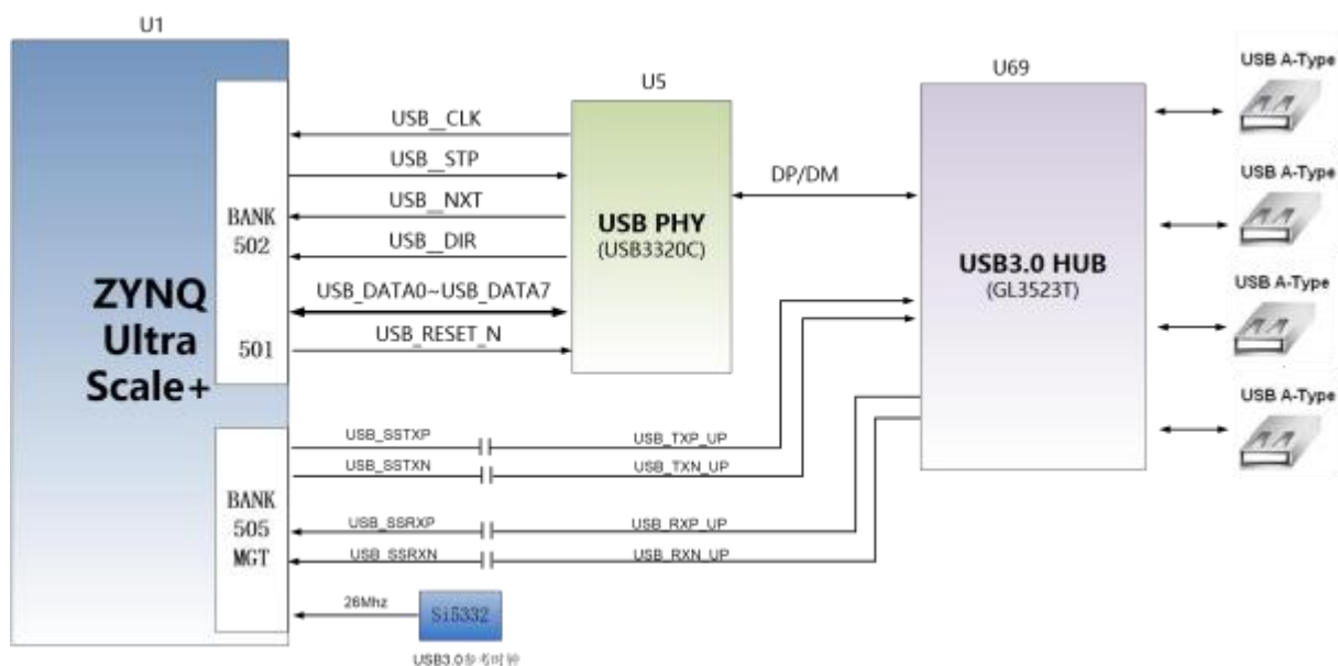
Figure 3-4-1: USB3.0 Interface Schematic
