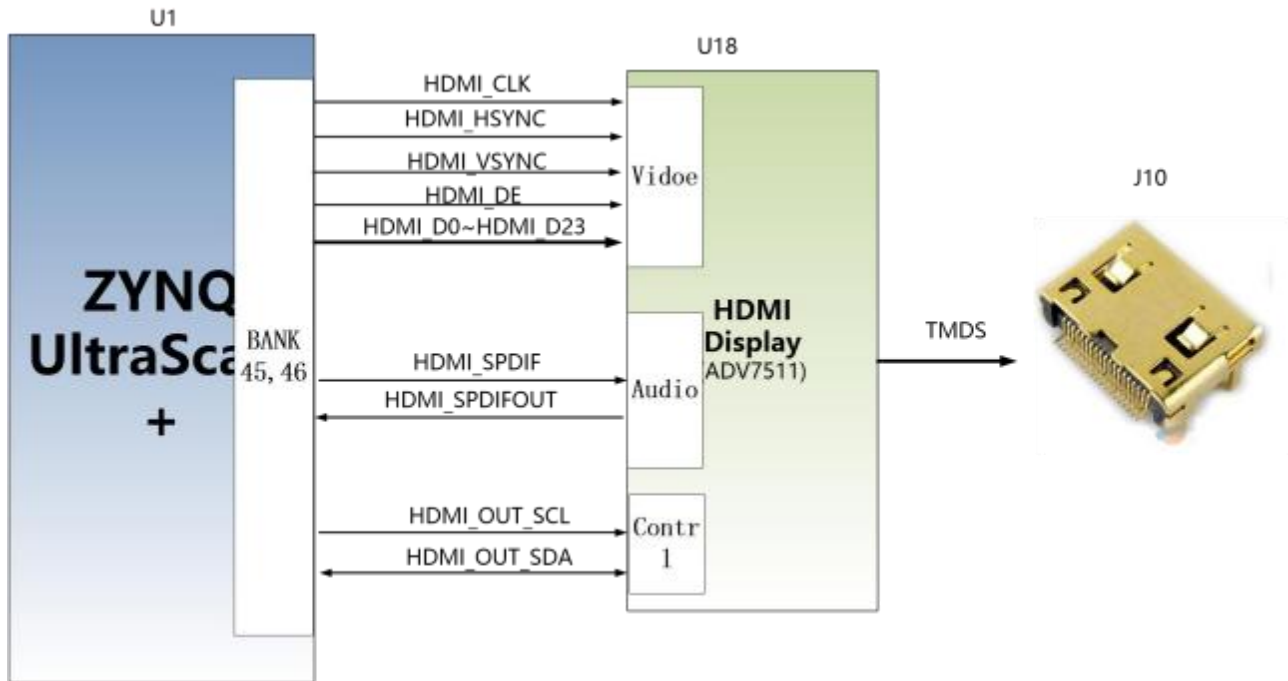
Figure 3-8-1: HDMI Output Interface Schematic
