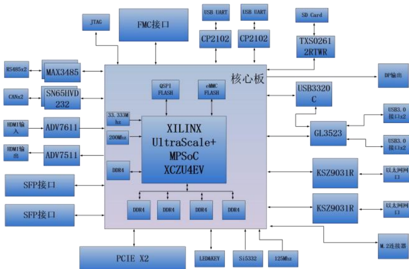
Figure 1-1-1: The Schematic Diagram of the AXU4EVB-P
