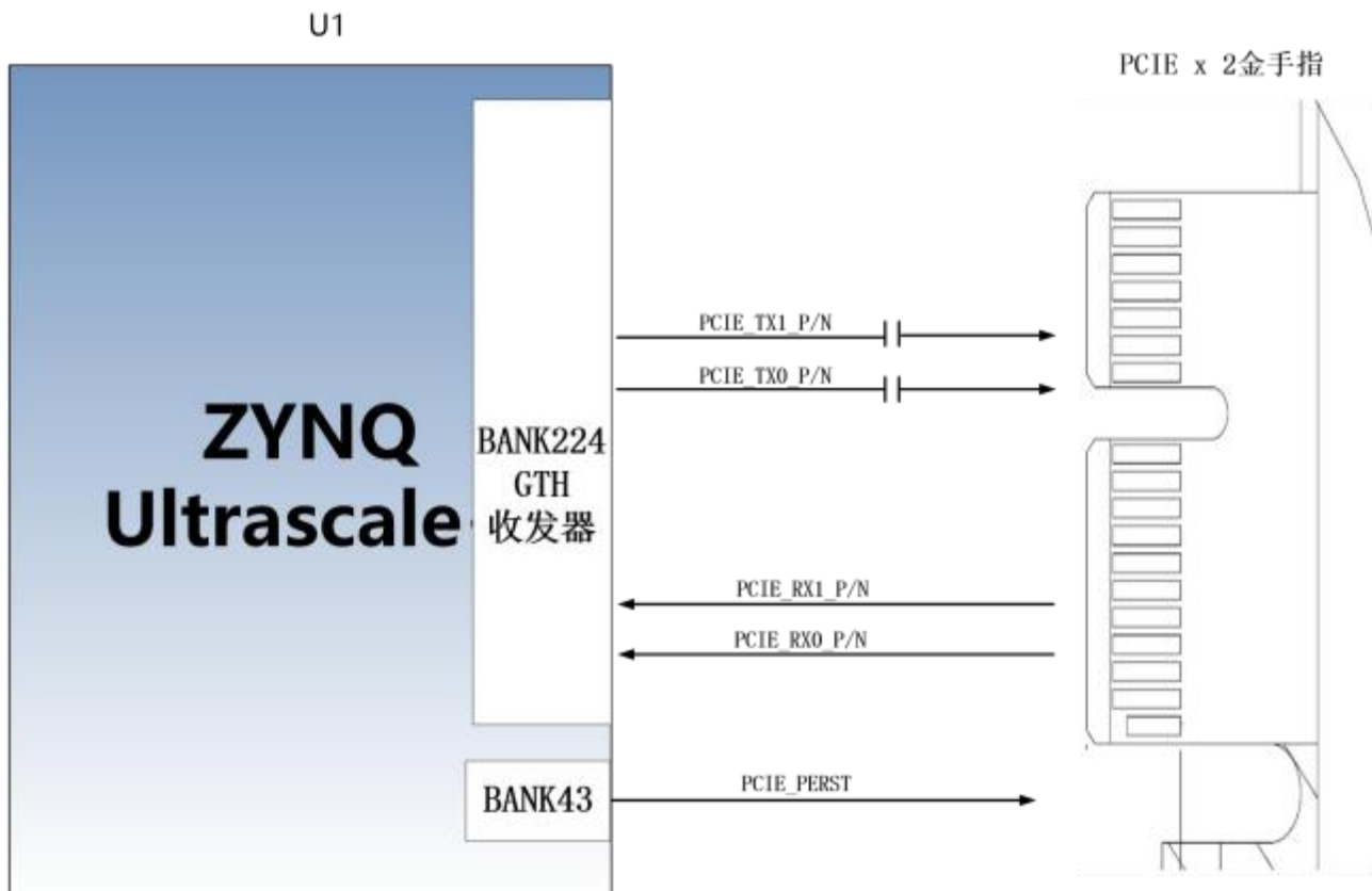
Figure 3-11-1: PCIe Interface Schematic
