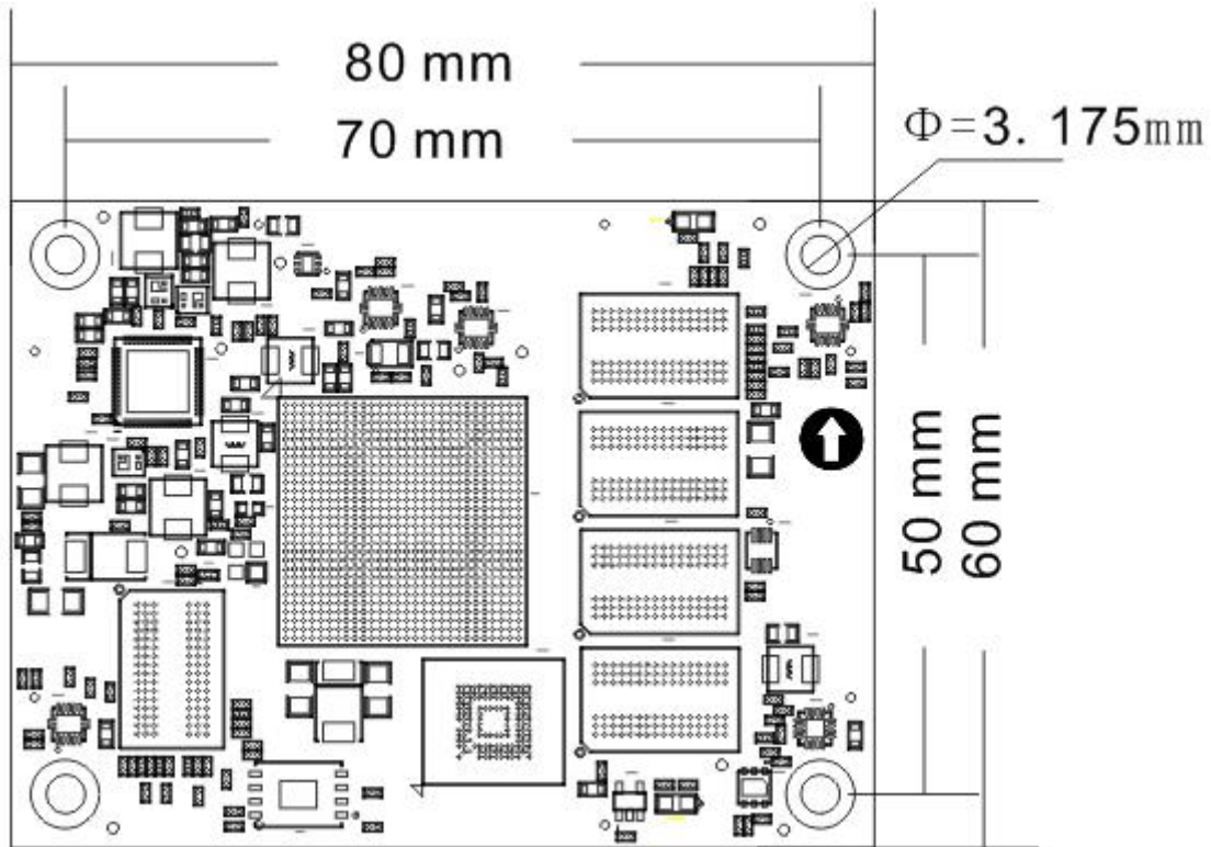
Figure 2-9-1: ACU5EVB-P Core Board Size Dimension
