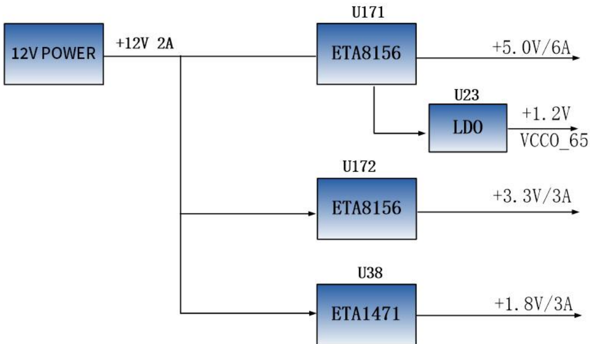
Figure 3-22-1: Carrier Board Power Schematic
