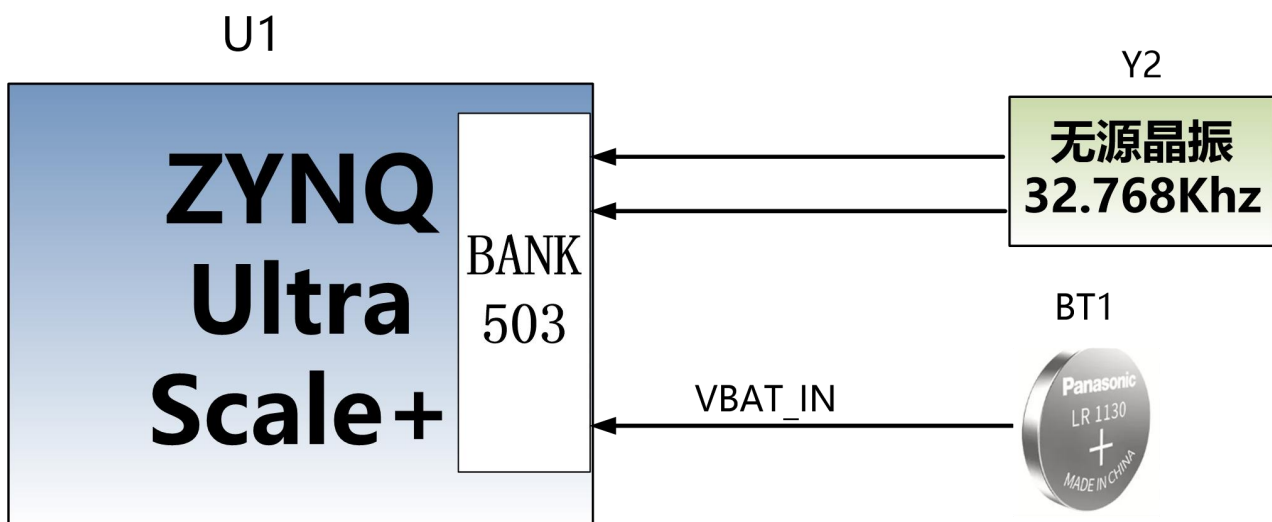
Figure 3-17-1: RTC Schematic
