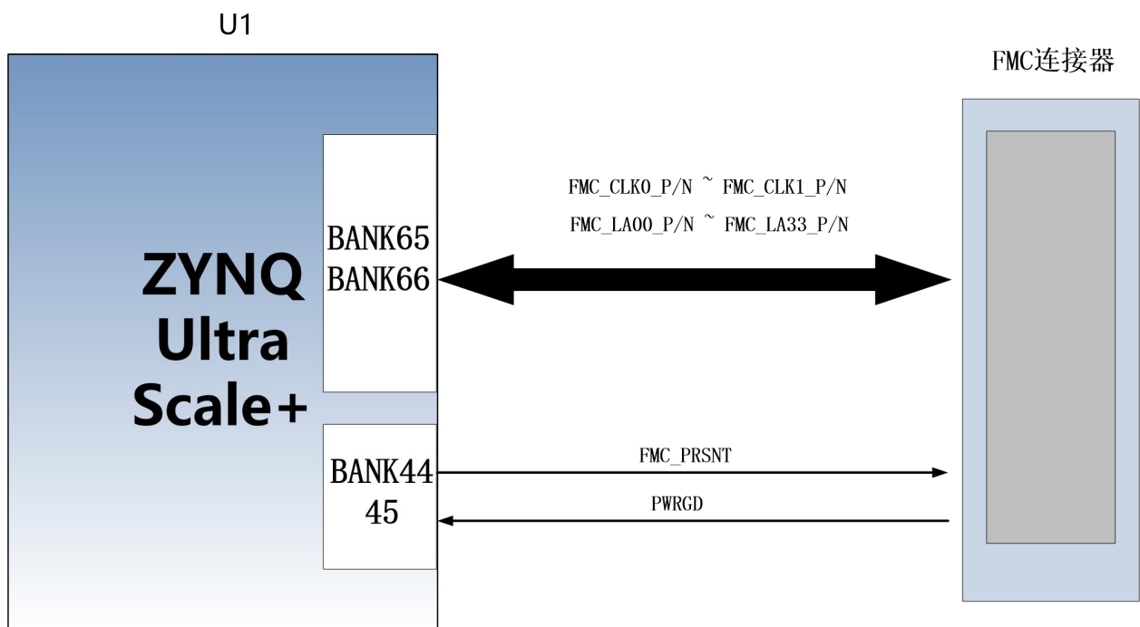
Figure 3-15-1: FMC Schematic
