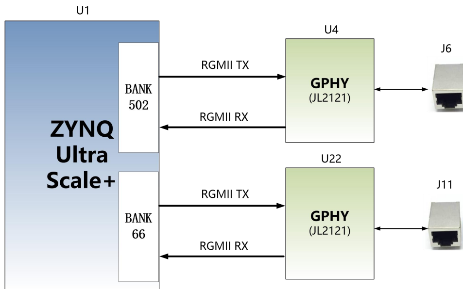
Figure 3-6-1: ZYNQ PS system and GPHY connection diagram
