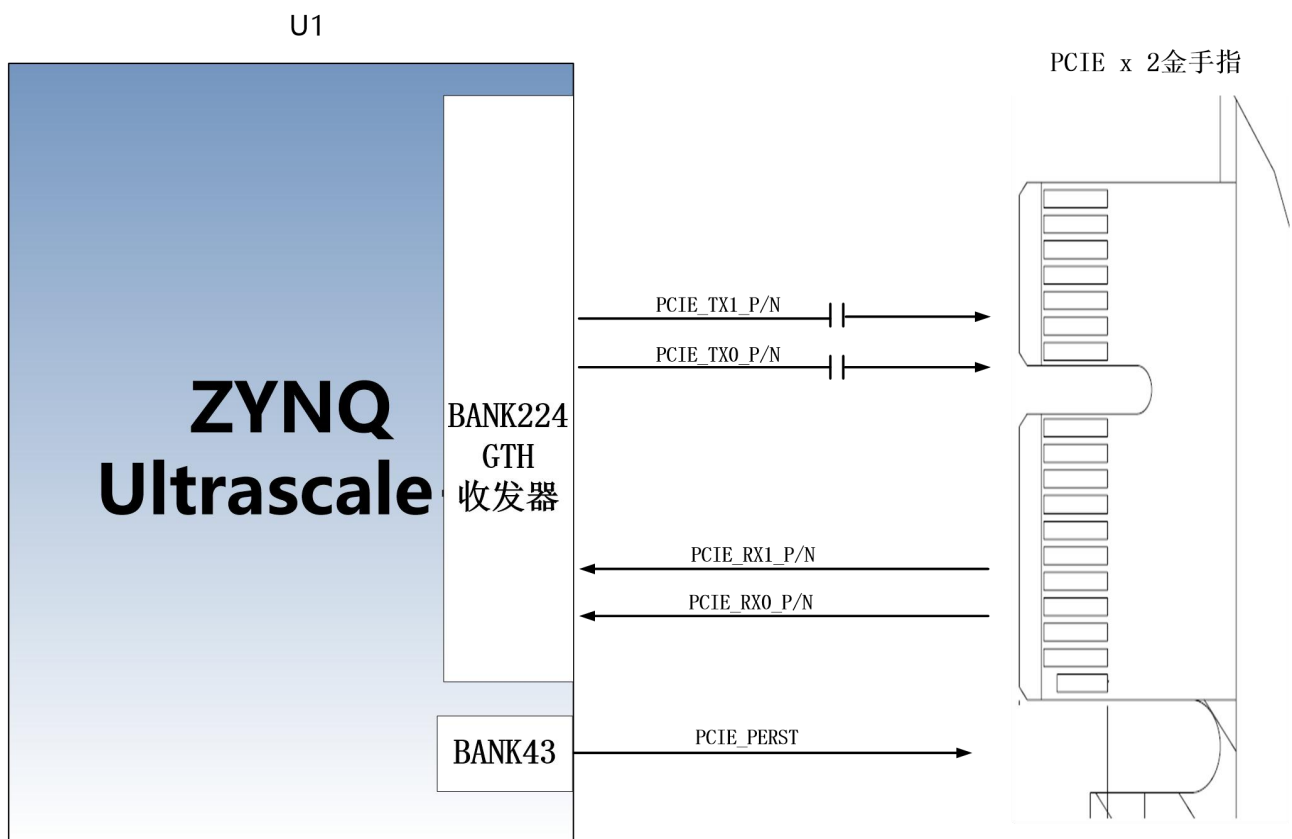
Figure 3-11: PCIe Interface Schematic
