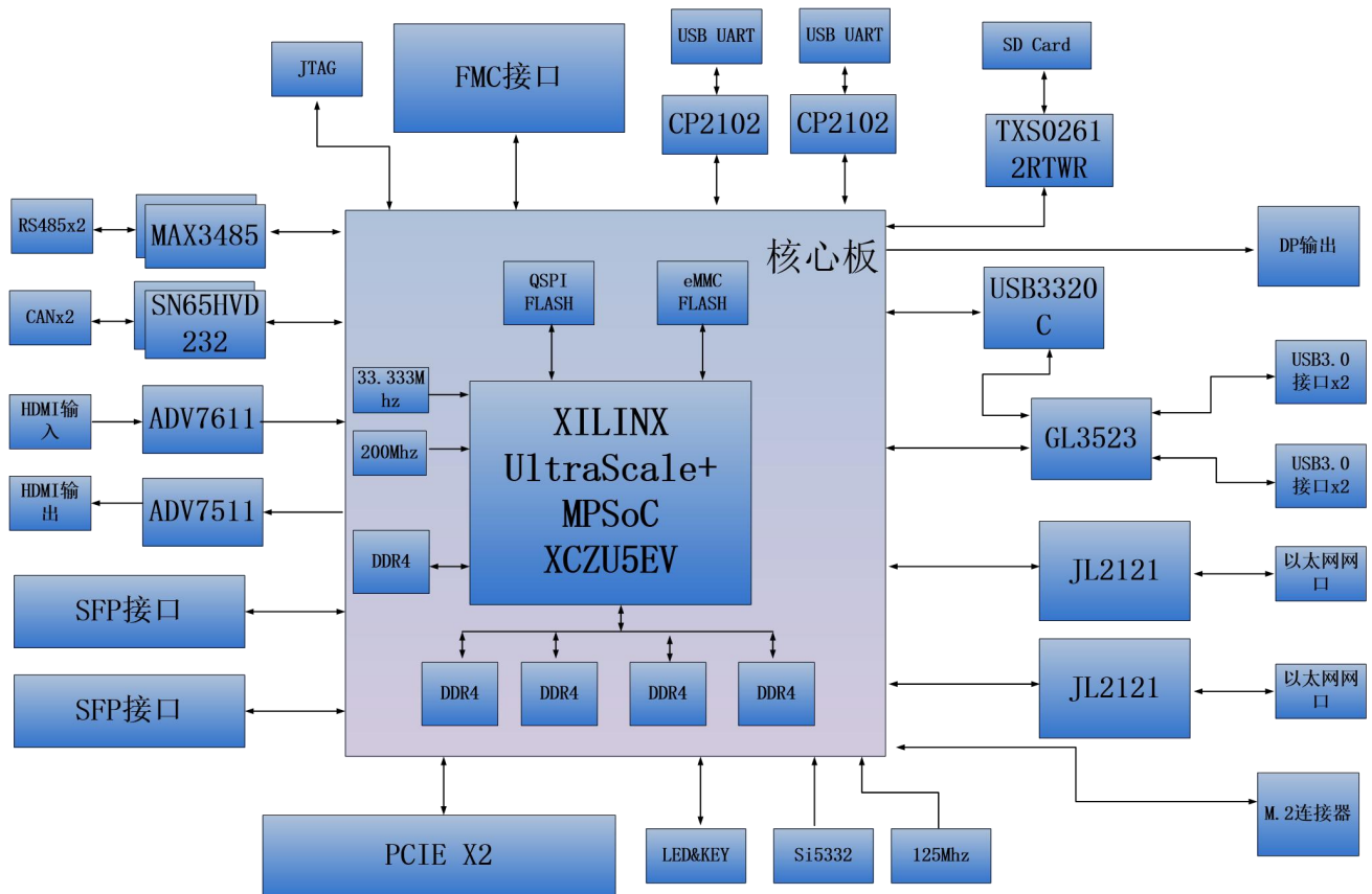
Figure 1-1-1: The Schematic Diagram of the AXU5EVB-P
