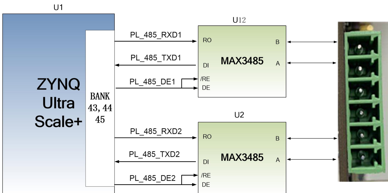
Figure 3-13-1: 485 Communication on the PL Side
