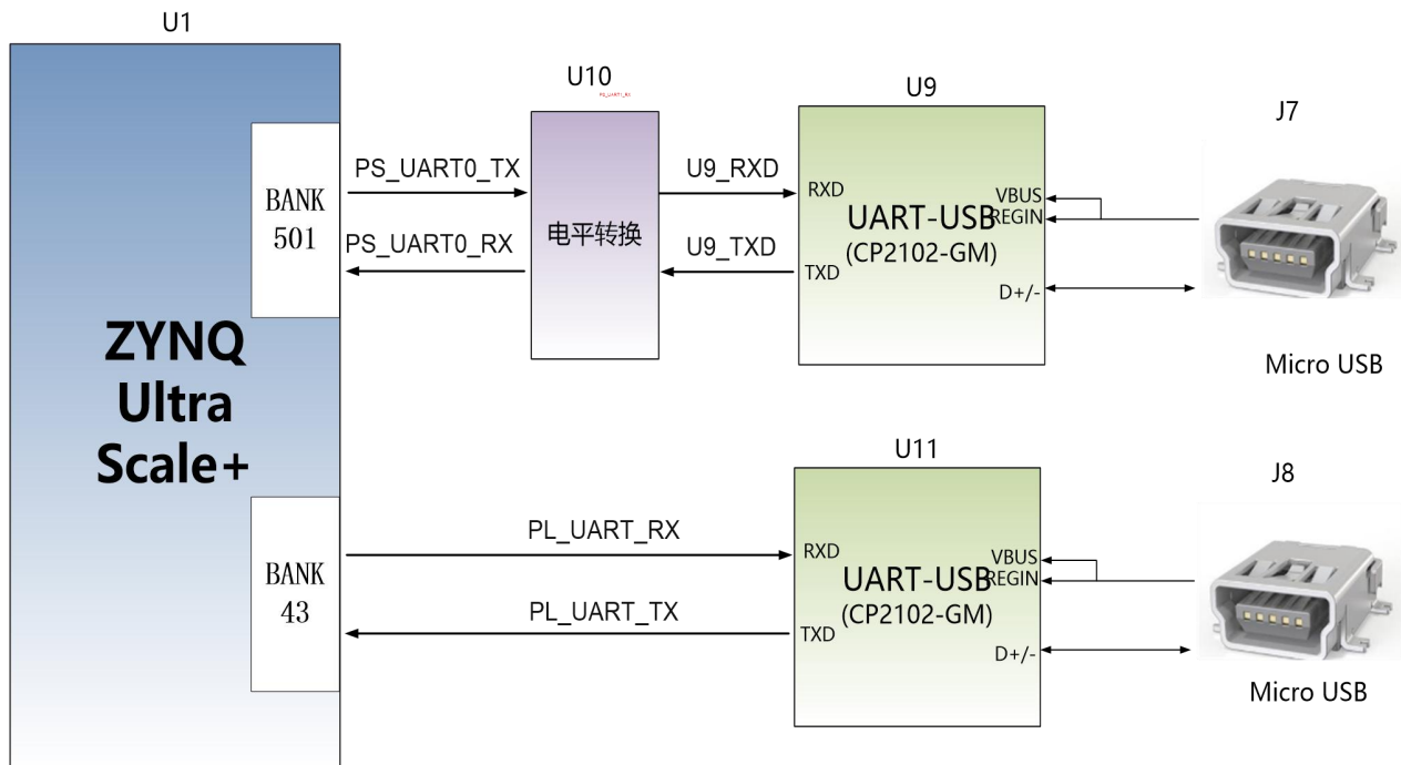
Figure 3-6-1: USB to serial port schematic
