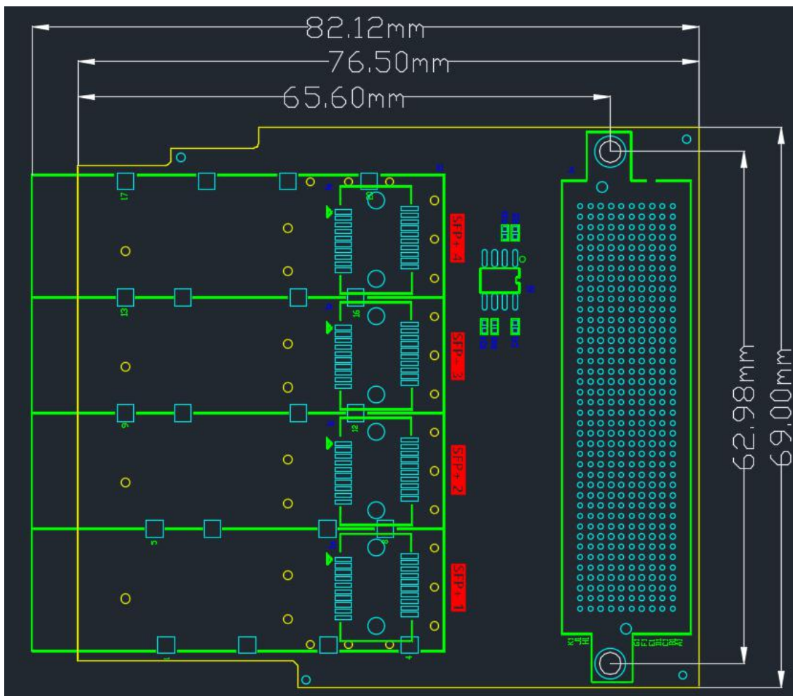
Figure 1-2: FH1223 Module Form Factor
