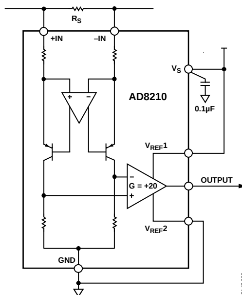
Figure 31. Split Supply
