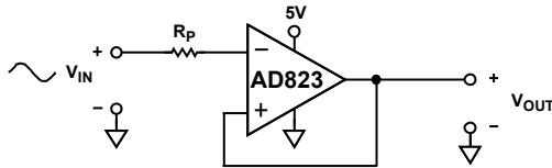
Figure 39. AD823 Input Response: V_{IN} = 0 to +V_S + 200 mV, V_{OUT} = 0 to +V_S , R_P = 49.9 k \Omega
