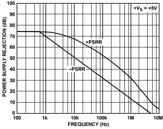
Figure 23. Power Supply Rejection vs. Frequency
