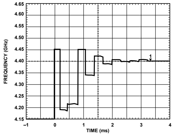
Figure 31. Lock Time for 250 MHz Jump from 4150 MHz to 4400 MHz, Loop Bandwidth = 20 kHz
