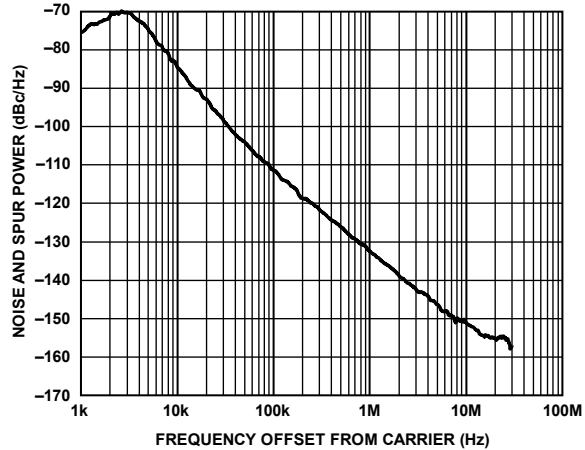
Figure 30. Fractional-N Spur Performance, R_{F_{OUTA+}} = 5.8 GHz, R_{F_{IN}} = 122.88 MHz, f_{PFD} = 61.44 MHz, Output Divide by 2 Selected, Loop Filter Bandwidth = 2 kHz, Channel Spacing = 20 kHz
