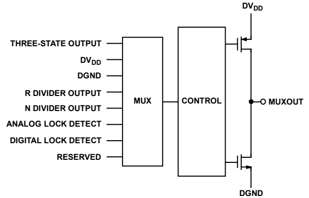
Figure 35. MUXOUT Schematic
