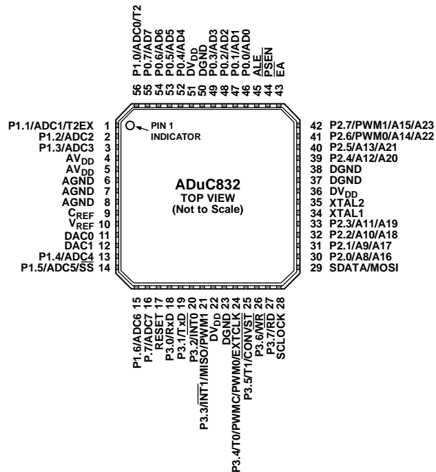
Figure 15. 56-Lead LFCSP
