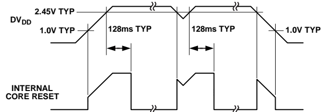
Figure 92. Internal POR Operation
