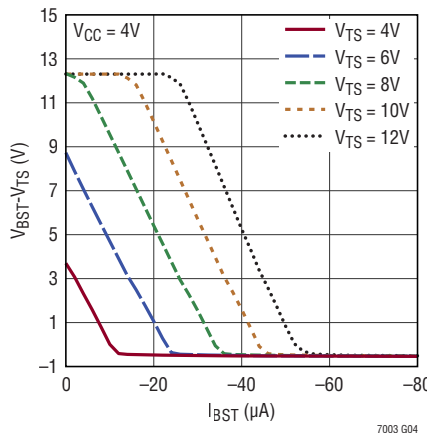
Charge Pump Load Regulation
