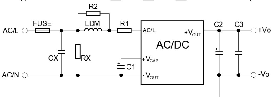
Figure 2. External circuit for EMC enhancement
