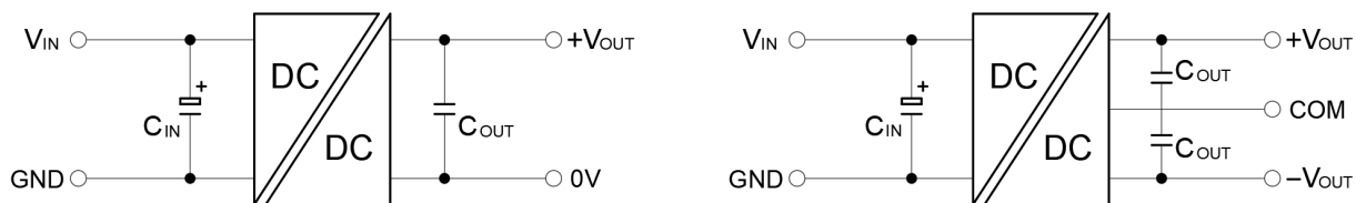
Figure 1. Typical Application Circuit
