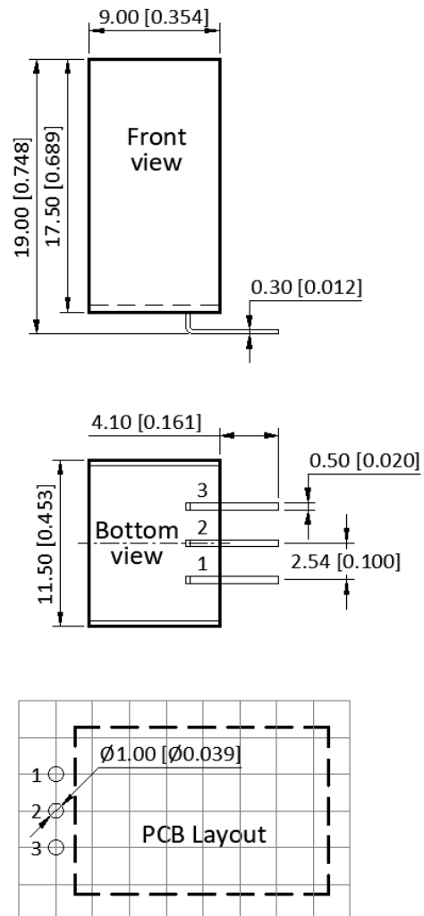
Suffix "L" Package
