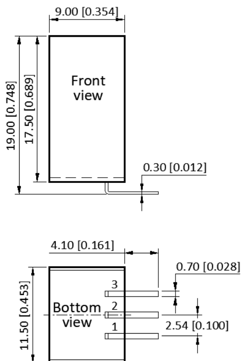
Suffix "L" Package
