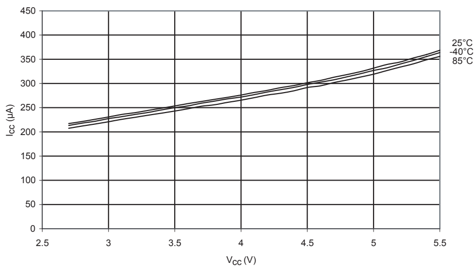
Figure 202. ADC Current vs. V_{CC} (AREF = AVCC)
