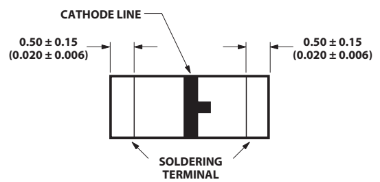
HSMx-C265
