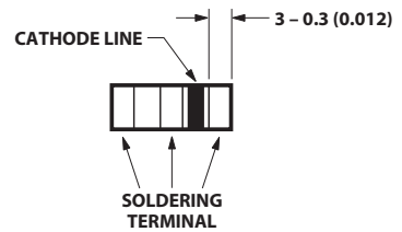
HSMx-C120
