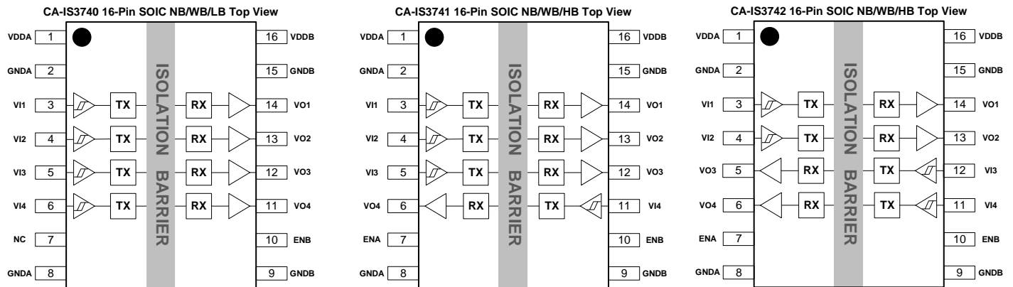
Figure. 6-1 CA-IS374x pin configuration
