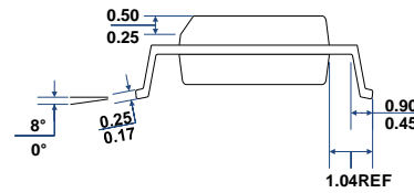
LEFT-SIDE VIEW
