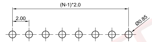
Recommended PCB Layout (Tolerance:±0.05)
