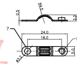
BIG WASHER
