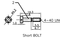
Short BOLT
