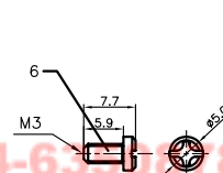
SHORT SCREW
