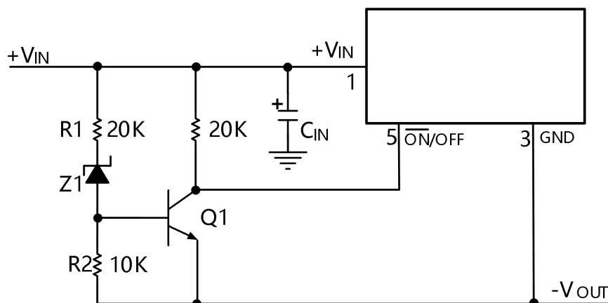
FIGURE 7. Undervoltage Lockout for Buck-Boost Circuit
