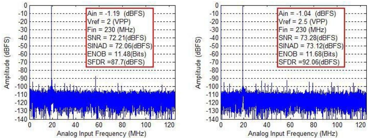
Figure 7. FFT characteristics: Analog input frequency 230MHz, sampling rate 250MSPS
