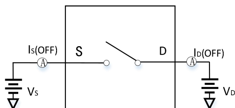
Figure 9. Off Leakage
