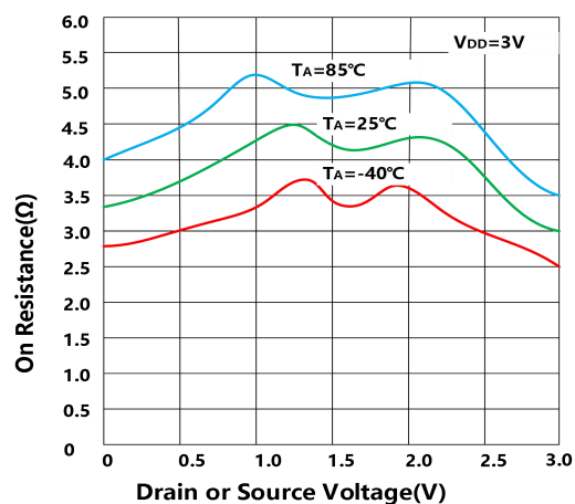
Figure 5. On Resistance vs. V_D ( V_S ) for Different Temperatures,
