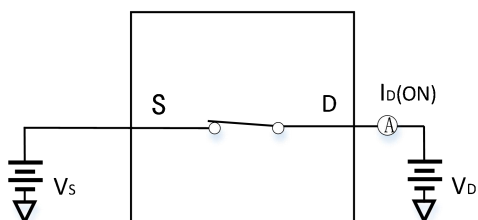
Figure 8. On Leakage
