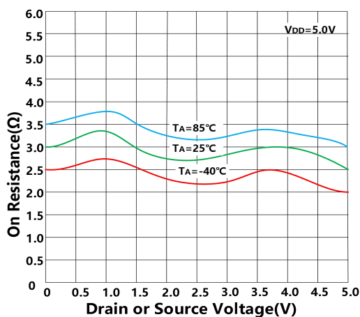
Figure 6. On Resistance vs. V_D ( V_S ) for Different
