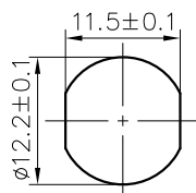
Panel Mounted
