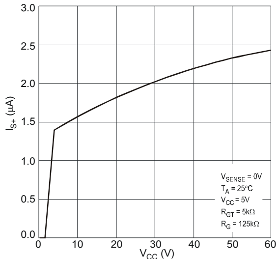
I_{S+} Input Current vs. V_{CC}
