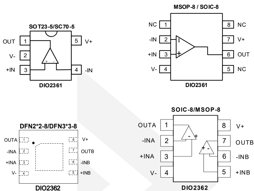
Figure 1 Top View
