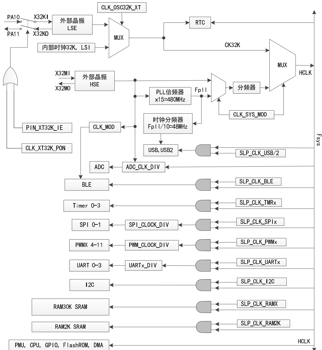
Figure 6-1 Clock tree block diagram
