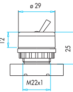
Mandallı Handle Button
