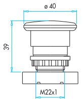
Mantar, Yaylı Mushroom, Spring Return
