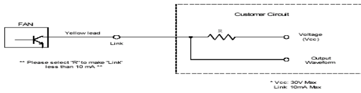
Speed Sensor / Tachometer ( FG/F )
