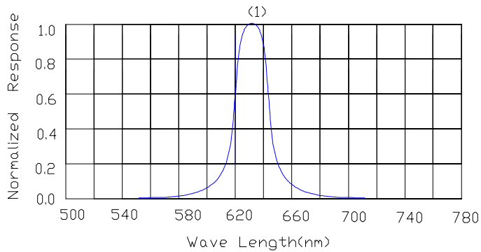
Spectral Reduance
