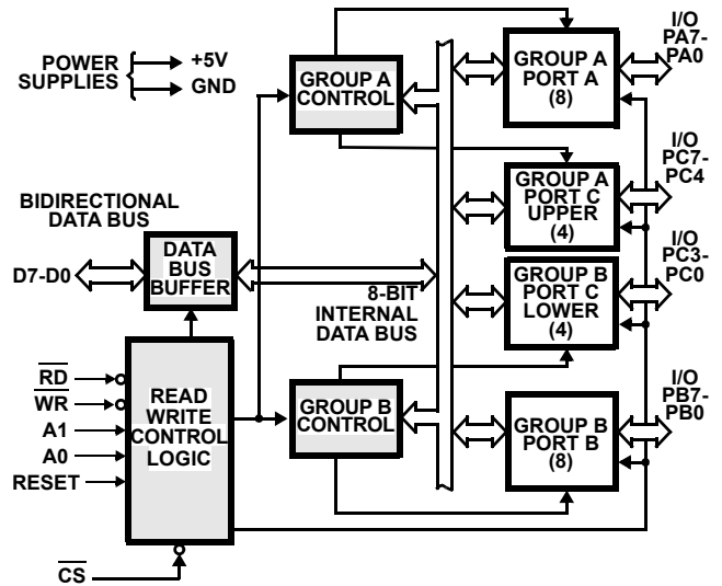
FIGURE 1. 82C55 BLOCK DIAGRAM. DATA BUS BUFFER, READ/WRITE, GROUP A & B CONTROL LOGIC FUNCTIONS
