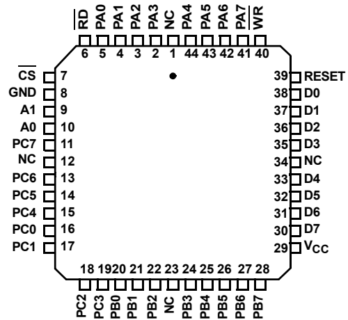
82C55 (PLCC) TOP VIEW
