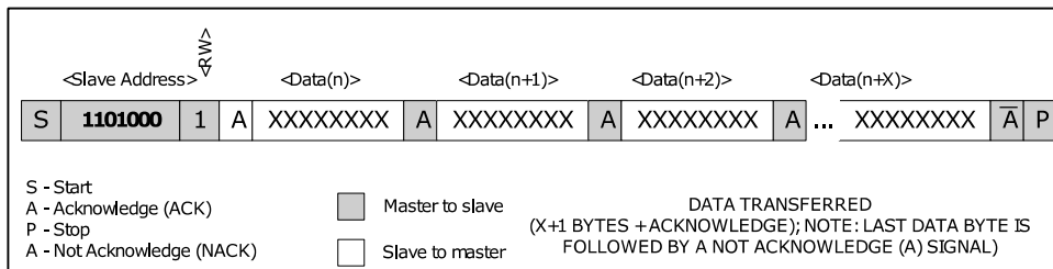
Fig. 2. Data Read—Slave Transmitter Mode
