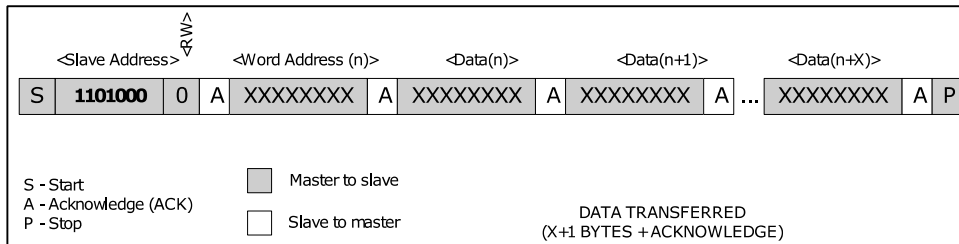
Fig. 1. Data Write—Slave Receiver Mode
