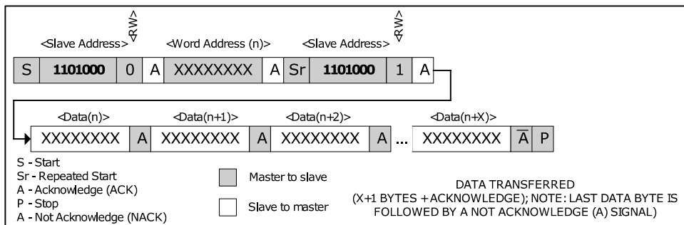
Fig. 3. Data Read (Write Pointer, Then Read)—Slave Receive and Transmit
