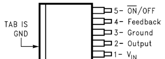
TO-263 (S) Top View
