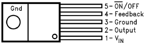
TO-220 (T) Top View
