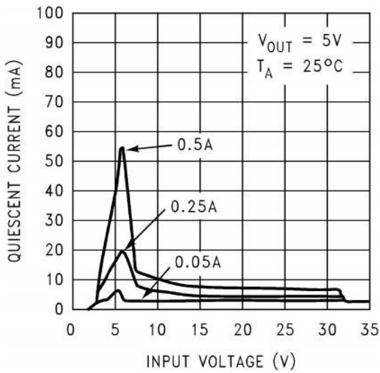
Fig 5. Quiescent Current vs. Input Voltage
