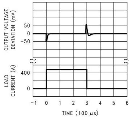
Fig 8. Load Transient Response
