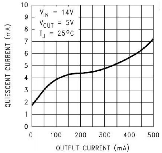
Fig 6. Quiescent Current vs. Output Current
