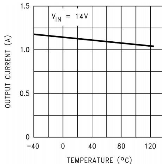
Fig 17. Peak Output Current
