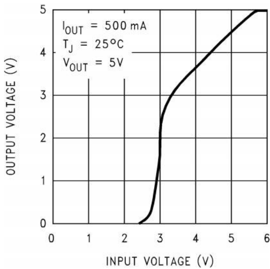
Fig 13. Low-Voltage Behavior
