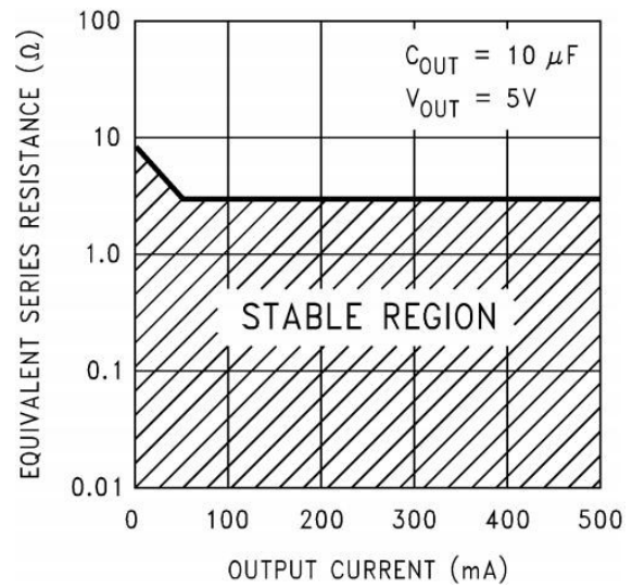
Fig 16. Output Capacitor ESR
