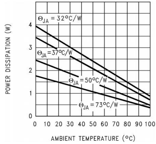
Fig 12. Maximum Power Dissipation (TO-263)
