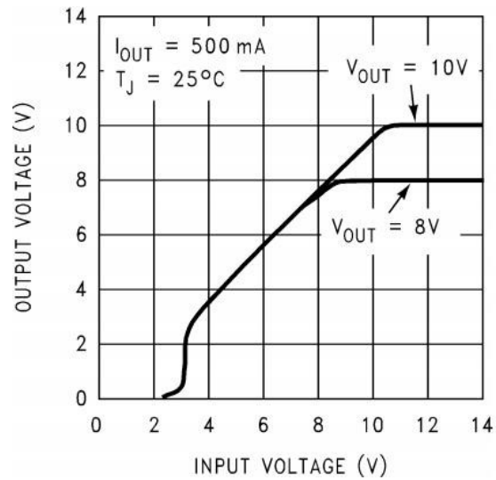
Fig 14. Low-Voltage Behavior
