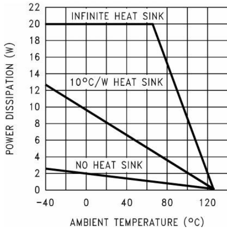
Fig 11. Maximum Power Dissipation (TO-220) 1
