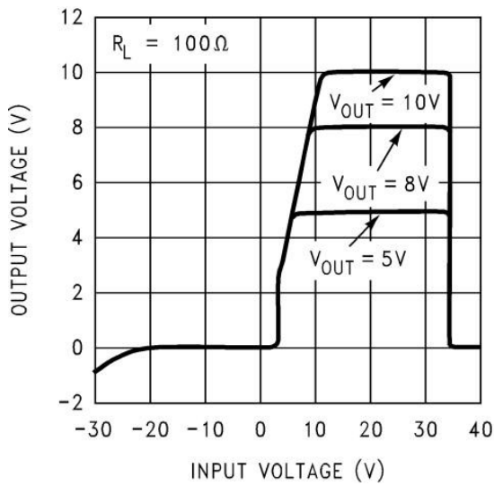
Fig 15. Output at Voltage Extremes
