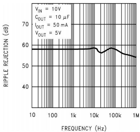
Fig 9. Ripple Rejection
