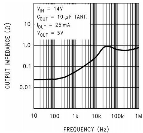
Fig 10. Output Impedance
