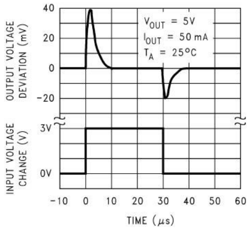
Fig 7. Line Transient Response
