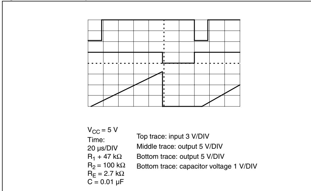
Figure 20. Linear ramp
