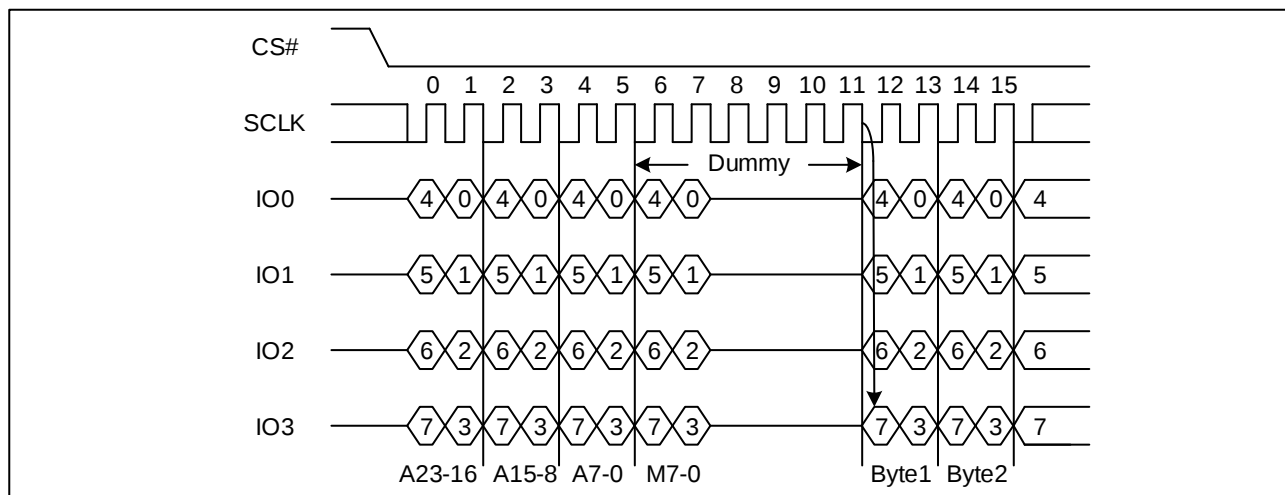
Figure 17. Quad I/O Fast Read Sequence Diagram ((M5-4) = (1, 0))
