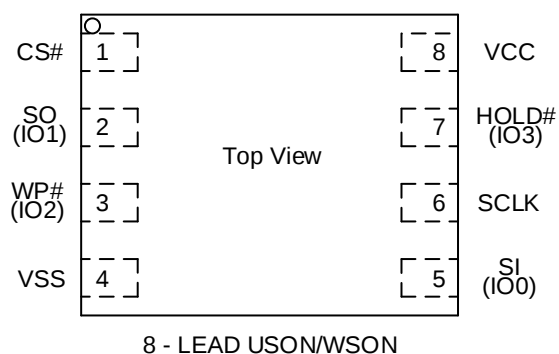
Figure 2 Connection Diagram for USON8/WSN8 Package
