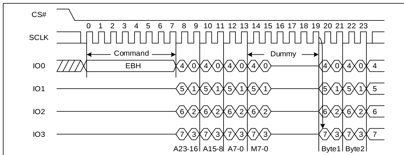
Figure 16. Quad I/O Fast Read Sequence Diagram ((M5-4) ≠ (1, 0))
